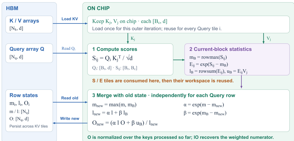
KV OUTER LOOP / SAME FOUR-ROW EXAMPLE · TWO QUERY TILES × TWO KV TILES
